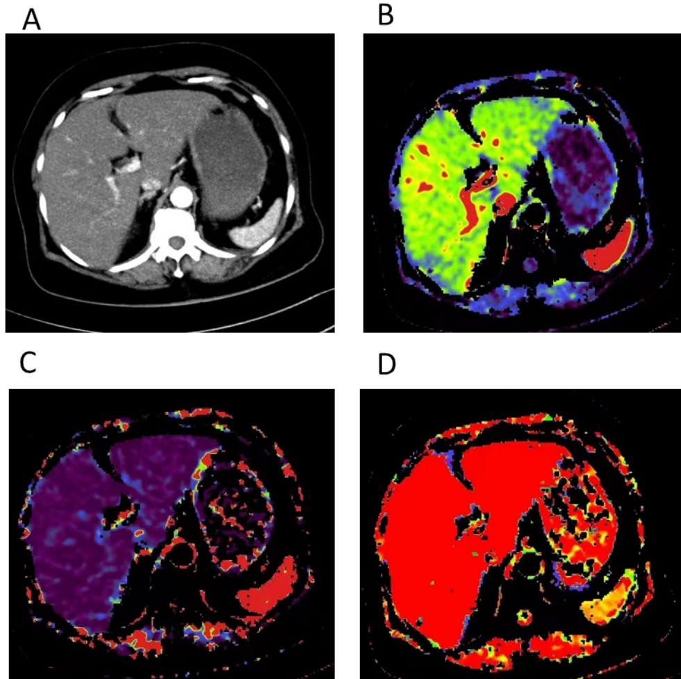
Fig 1. Plain and enhanced CT images of A patient with hepatocellular carcinoma (A) The original image showed A huge lesion in the right lobe of the liver with significantly uneven enhancement. (B) HAC images showed heterogeneous hyperperfusion. (C) PVC images showed hypoperfusion. (D) AEF images showed heterogeneous hyperperfusion throughout the lesion.
